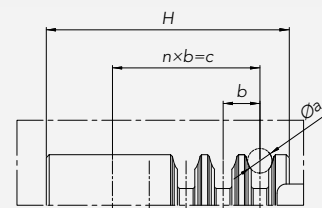
DETAL Z-Z (4:1)
